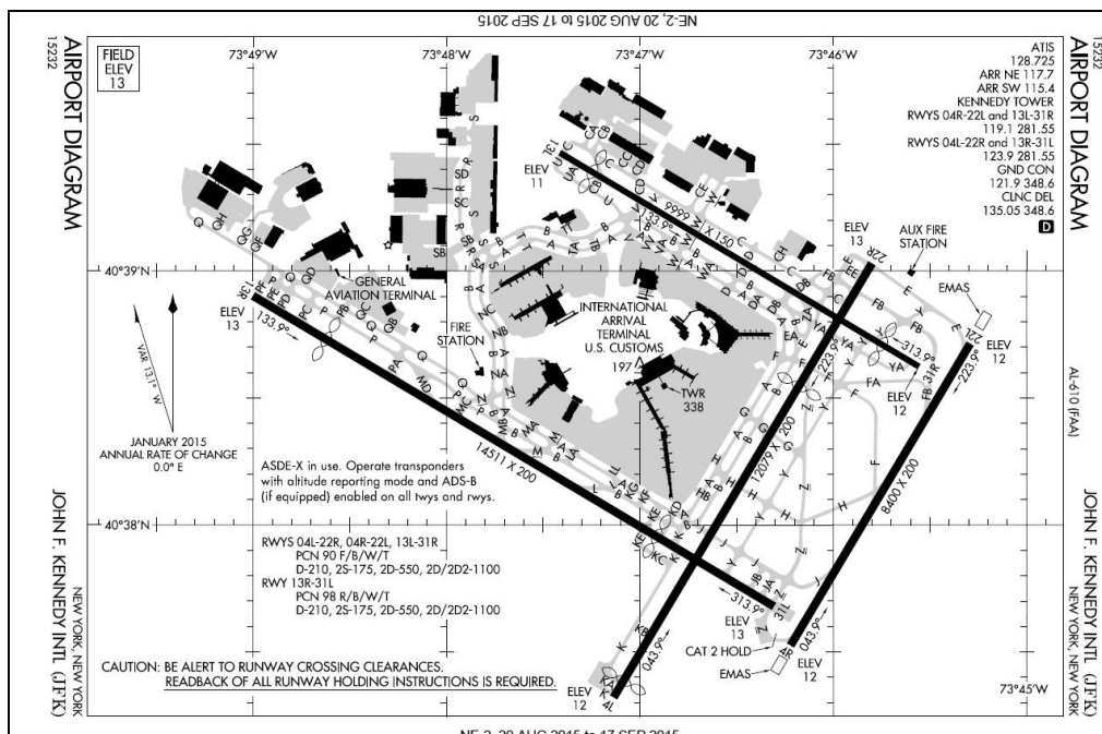
Figure 1: Airport diagram for John F. Kennedy
