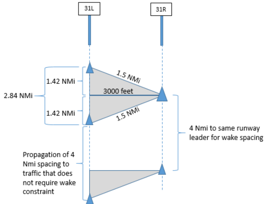
Figure 5: 1.5 mile stagger impact
